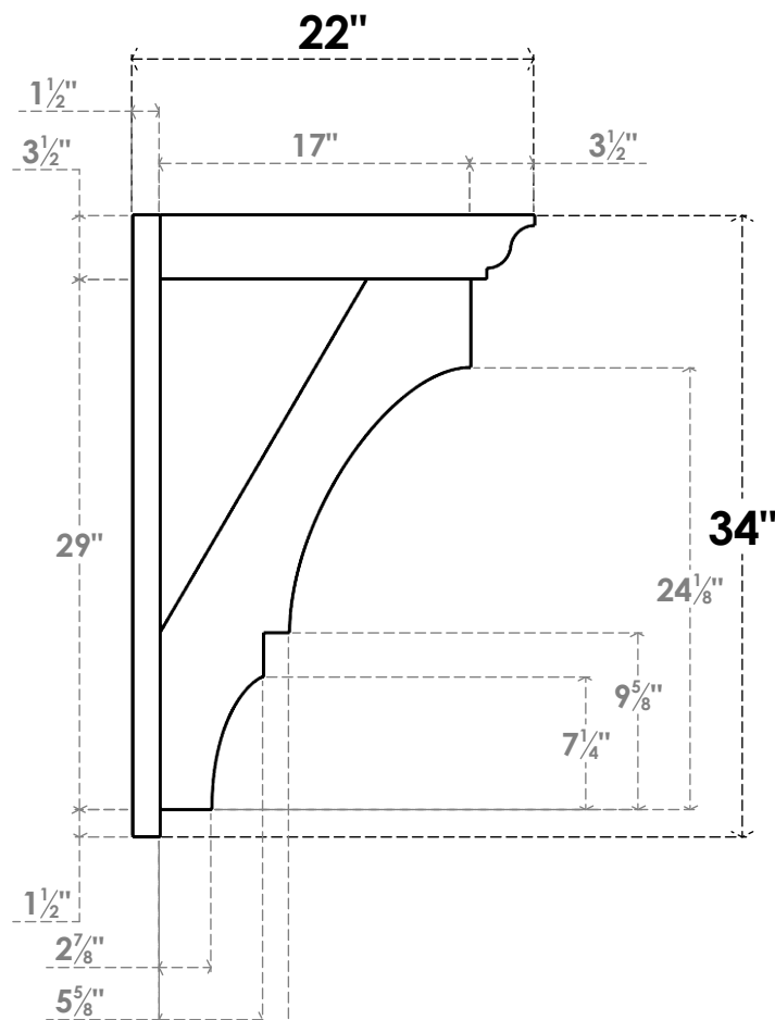
SIDE PROFILE
